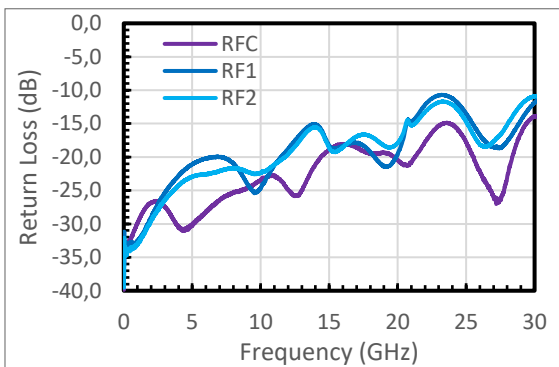
Figure 6 - Return Loss.
