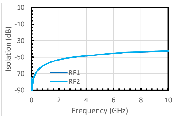
Figure 8 - Isolation (DC-10 GHz).
